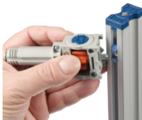
Captured sliding thread inserts can't get lost!
